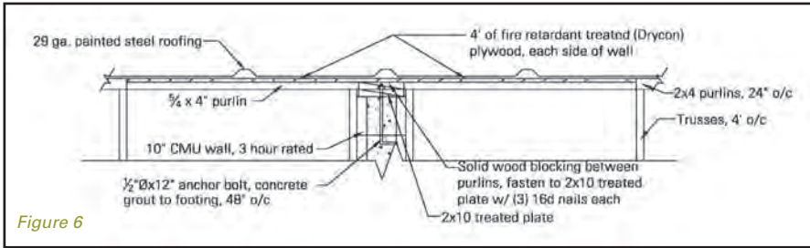
Figure 6. Detail for top of CMU wall termination.
